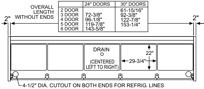
PLAN VIEW
