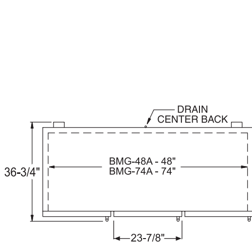
PLAN VIEW
