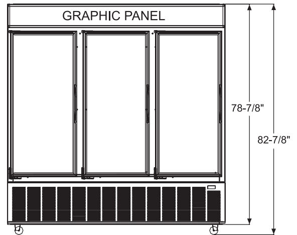
ELEVATION VIEW
