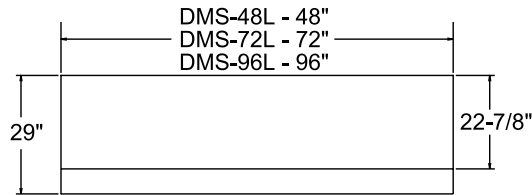
PLAN VIEW
