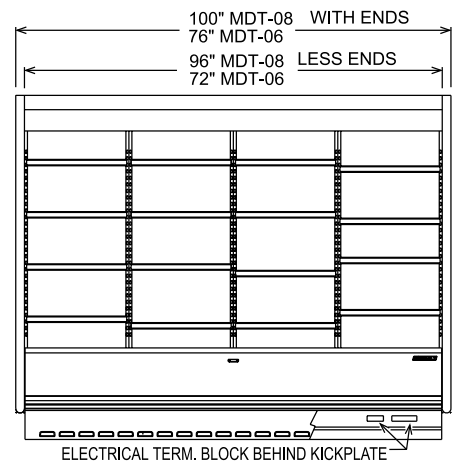
ELEVATION VIEW
