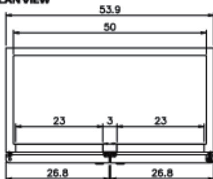
TWO DOOR PLAN VIEW
