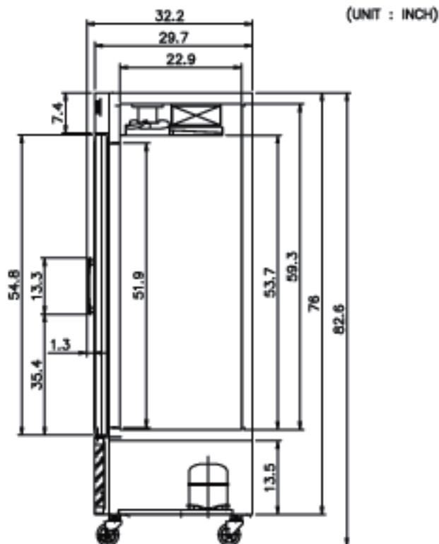
GLASS DOOR REACH-IN REFRIGERATOR SIDE VIEW
