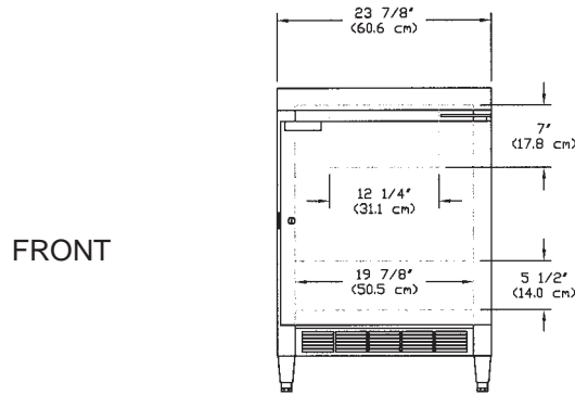
NSLR041WMW/0 - Forced Air Model
