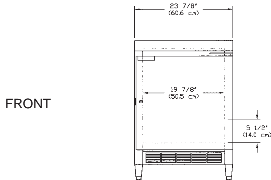
NSLR041WMW/0M - Cold Wall Model
