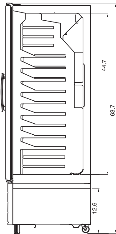
TGM-11R SIDE VIEW
