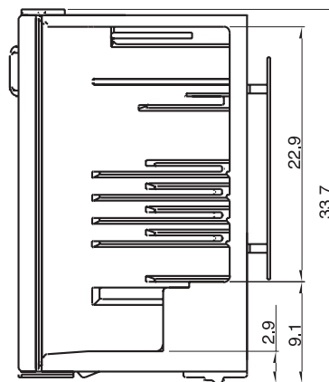
TGM-5R SIDE VIEW
