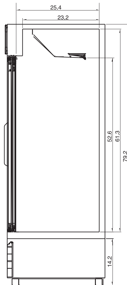
TGM-69R SIDE VIEW
