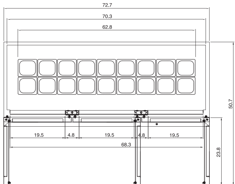
TST-72SD PLAN VIEW
